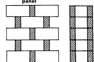
20 Cavity wall of 2x1/4 brick leaves bonded by header bricks on edge
